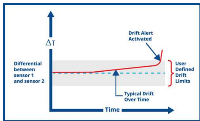
Figure 3-22: Thermocouple Degradation Diagnostic Detects a Degrading Thermocouple
