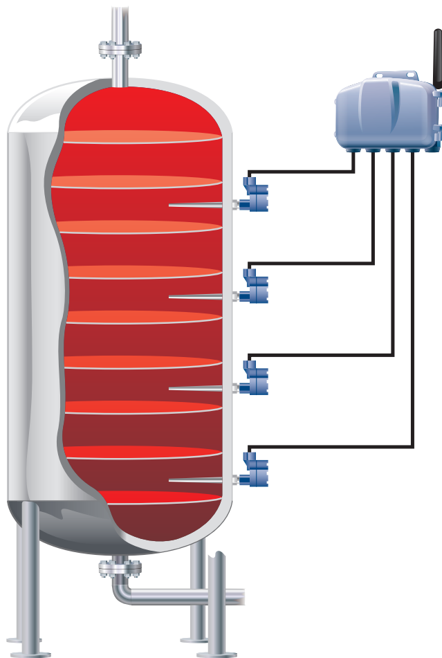
Figure 3-6: Temperature Profiling a Reactor
