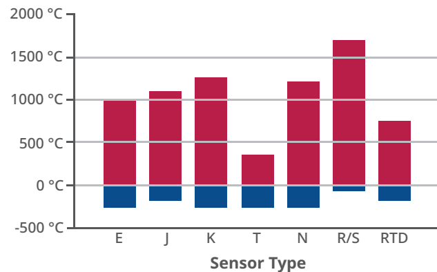
Figure 4-12: Potential Sensor Ranges in ^{\circ}\text{C}
