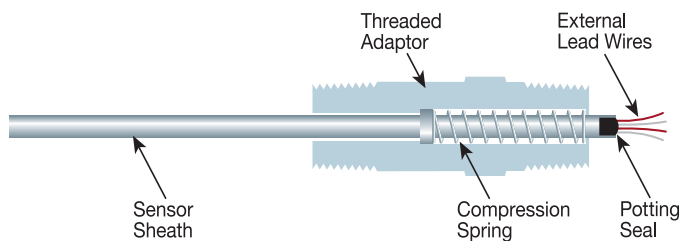
Figure 3-49: Spring-Loaded Threaded Style
