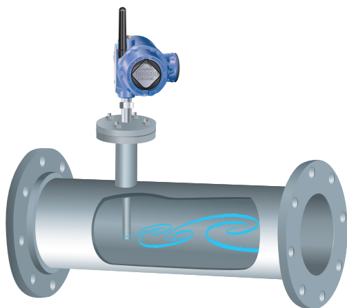
Figure 3-12: Wireless Remote Mount Pipeline Installation
