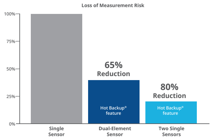
Figure 3-20: The Hot Backup Feature Prevents Primary Sensor Failure from Disrupting Process Control
