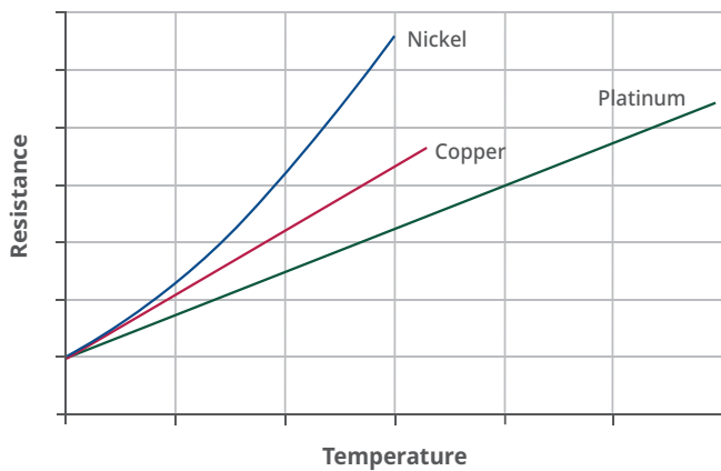
Figure 3-39: Resistance Changes vs. Temperature for Common Sensor Materials
