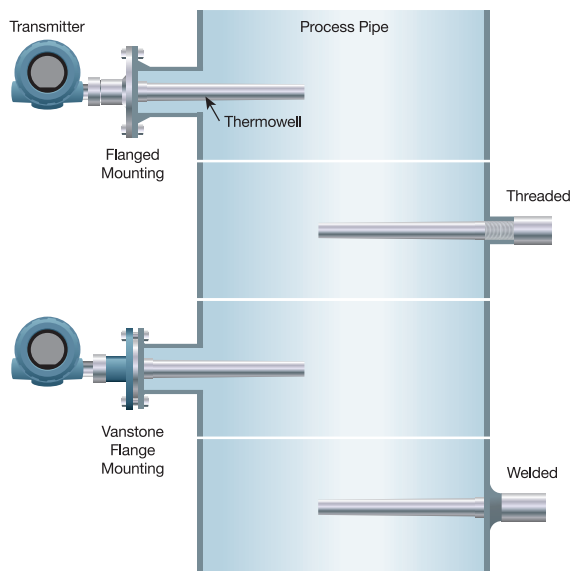
Figure 3-89: Thermowell Mounting Methods
