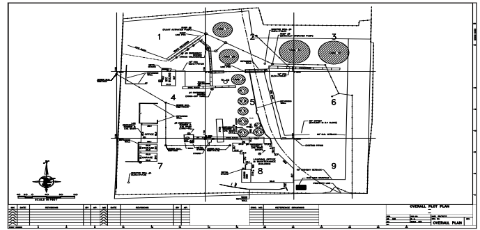
Figure 4-38: Typical Plot Plan
