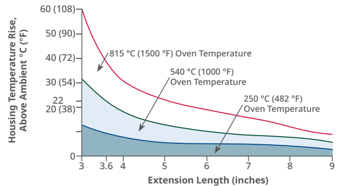
Figure 4-22: Transmitter Housing Temperature Rise vs. Extension Length for a Test Installation
