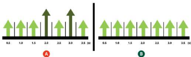
Figure 3-17: Output Without Transient Filtering (A) and With Transient Filtering (B)
