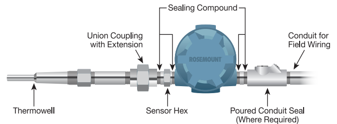
Figure 4-32: Typical Mounting with Drain Seal
