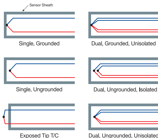
Figure 3-73: Hot Junction Configurations
