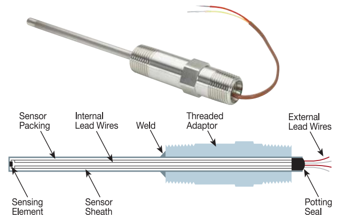
Figure 3-48: General Purpose Welded Adapter Style
