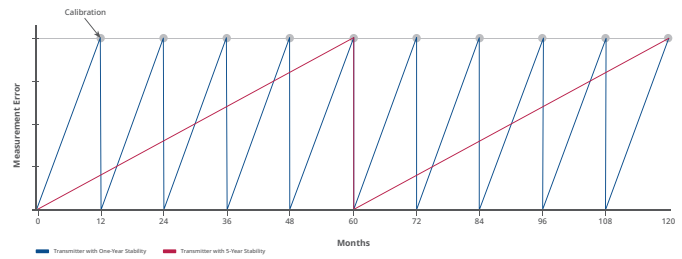
Figure 3-15: Comparing Transmitters with One-Year Stability vs. Transmitters with 5-Year Stability
