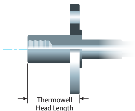
Figure 3-90: Thermowell Head Length
