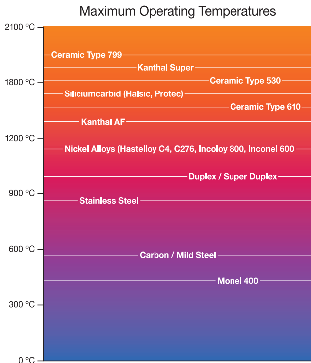
Figure 3-82: Thermowell Material Recommendations
