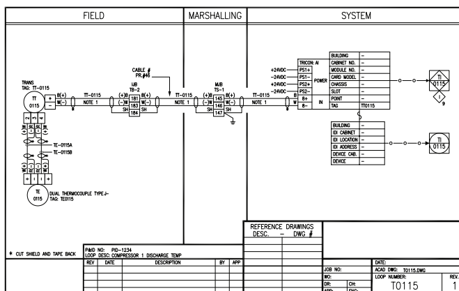
Figure 4-43: Typical Loop Sheet
