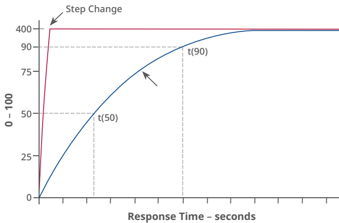
Figure 3-58: Typical Sensor Response Time
