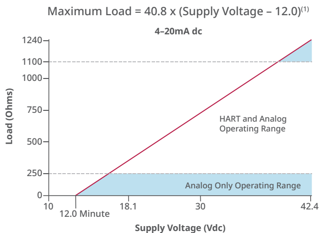
Figure 4-48: Loop Loading
