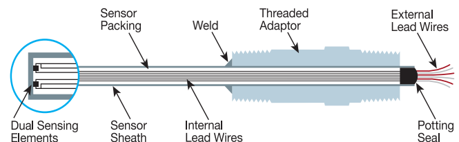
Figure 3-42: Dual Element RTD
