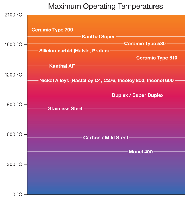
Figure 4-3: Maximum Temperatures of Thermowell Materials
