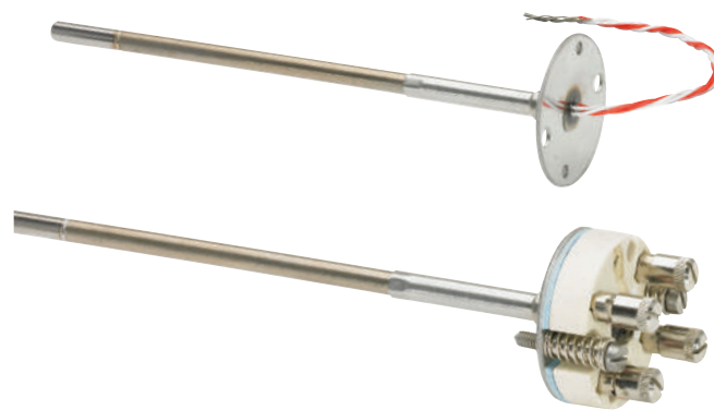
Figure 3-51: DIN Mount Sensors – Flying Leads – Terminal Block
