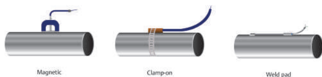
Figure 3-98: Temperature Measurement Installation Examples
