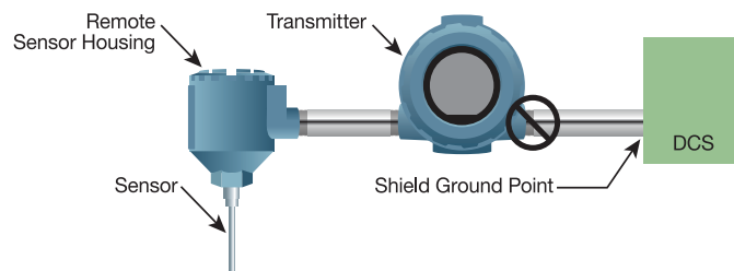
Figure 4-36: Option #2 for Shield Grounding
