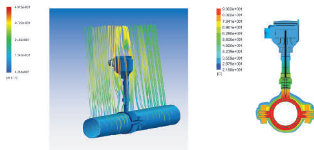
Figure 3-100: Free Convection Model
