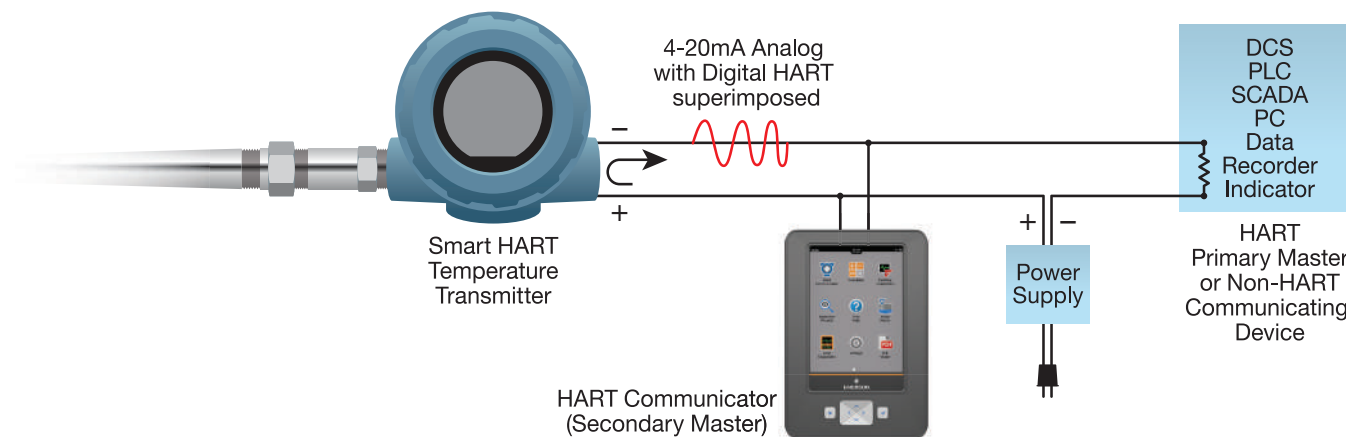
Figure 3-10: HART Device Connection
