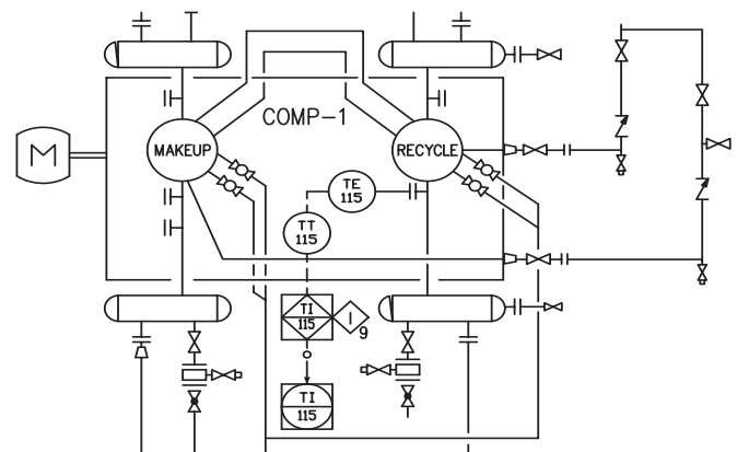
Figure 4-40: Example of a P&ID
