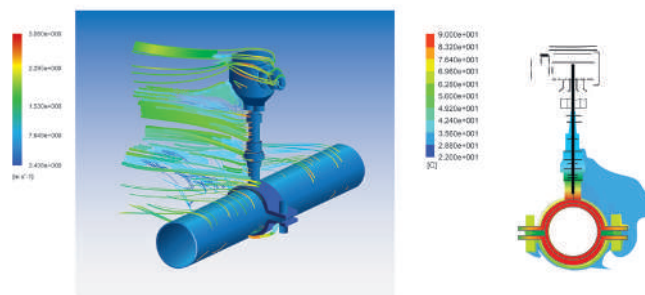
Figure 3-101: Forced Convection Model
