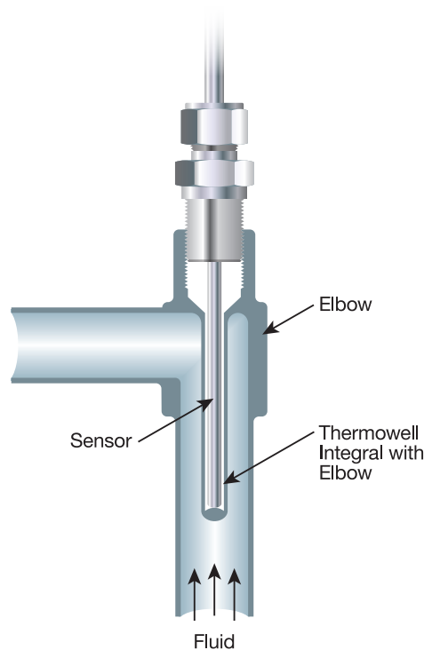
Figure 4-5: Thermowell Elbow Installation
