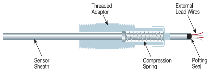
Figure 3-50: Bayonet Style Spring-Loaded Sensor Assembly
