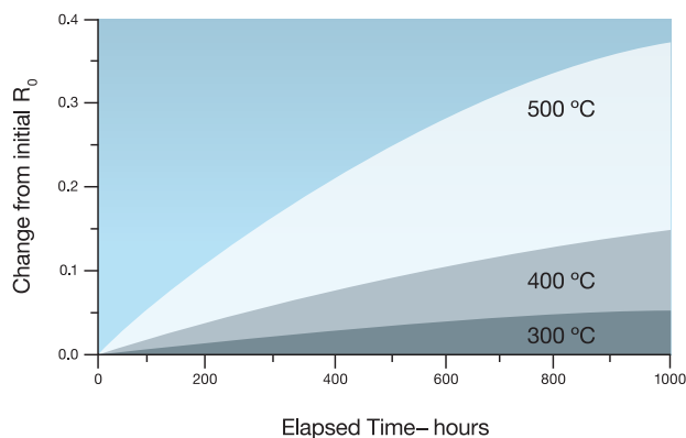
Figure 3-69: Shift of R_0 vs. Time vs. Temperature
