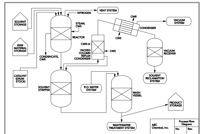
Figure 4-39: Typical Process Flow Diagram
