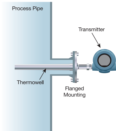
Figure 3-53: Transmitter Assembly Pipeline Installation
