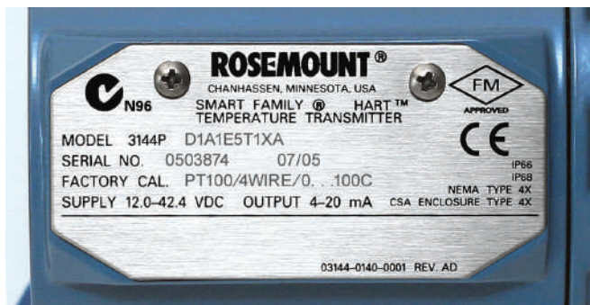
Figure 3-37: Standard Instrument Tag
