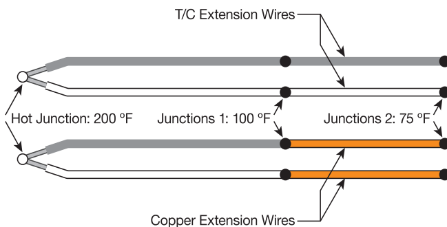
Figure 3-77: Multiple Junctions Caused by Non-Similar Extension Wire
