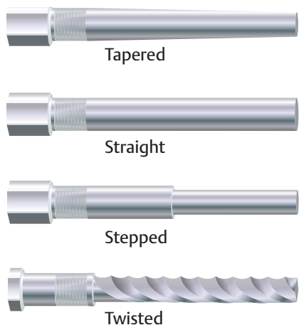
Figure 3-84: Thermowell stem profiles
