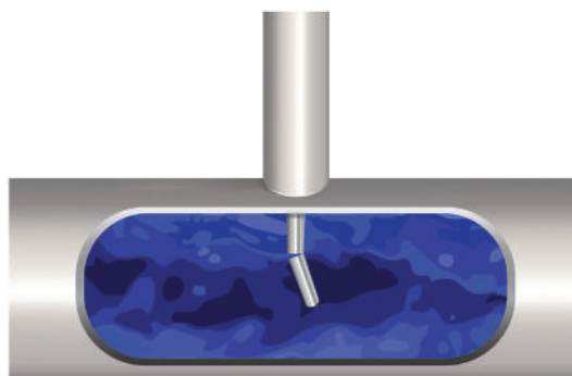
Figure 3-97: Thermowell Breakage due to Fatigue caused by Internal Process Fluid Velocity and Ultimately, Failure of the Thermowell.
