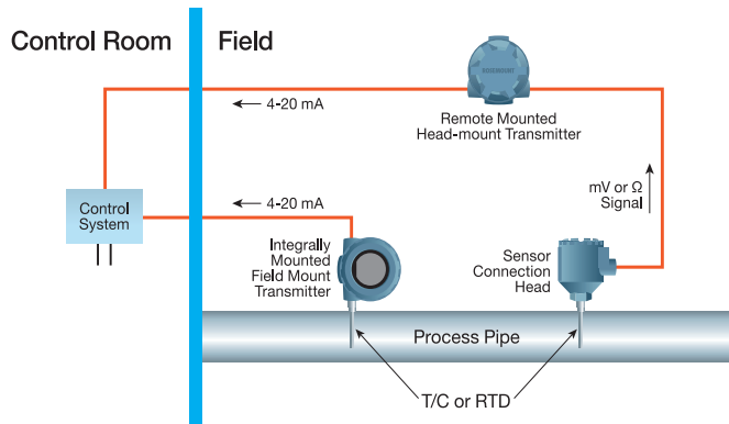
Figure 3-29: Integral Mount vs Remote Mount Configurations
