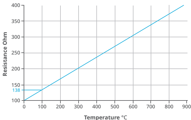
Figure 3-57: Temperature Coefficient of Resistance (TCR) of a Pt100 RTD
