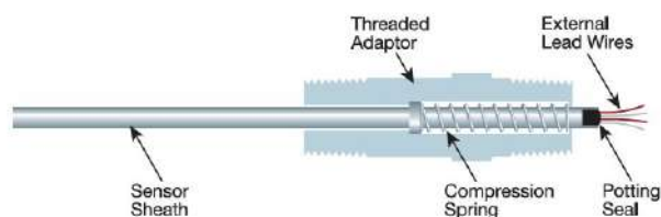
Figure 6-2: Spring-Loaded Sensor
