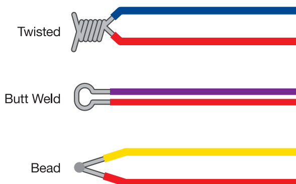
Figure 3-72: Hot Junction Methods
