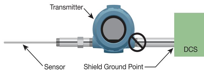
Figure 4-37: Option #3 for Shield Grounding
