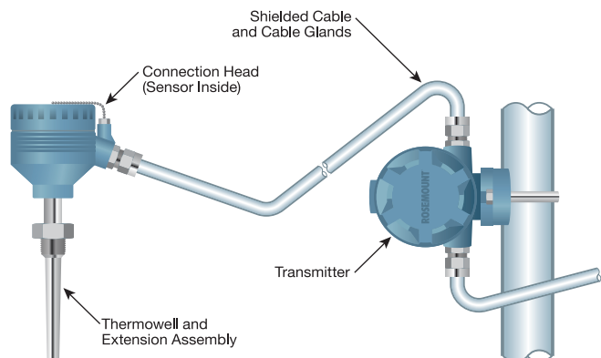
Figure 4-34: Typical European Mounting
