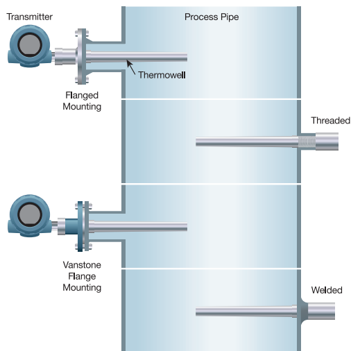
Figure 4-4: Thermowell Mounting Methods
