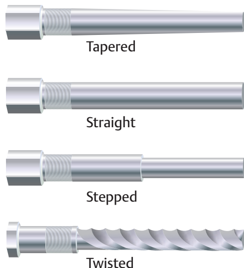
Figure 4-10: Thermowell stem profiles
