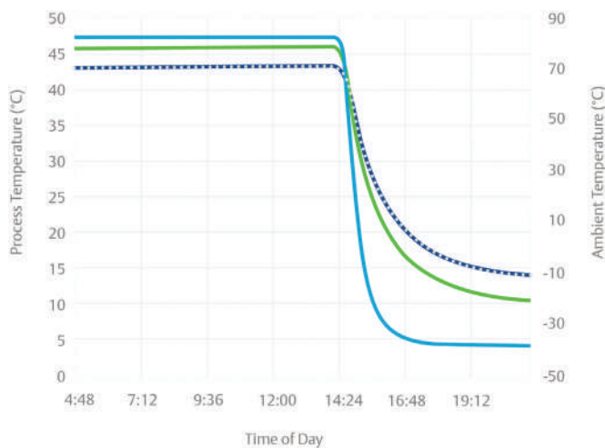
Figure 3-106: Correction Applied to Changing Ambient Temperature: Insulated Surface Sensor and Inserted RTD Sensor Comparison (1-in. Carbon Steel Schedule 40 Pipe)
