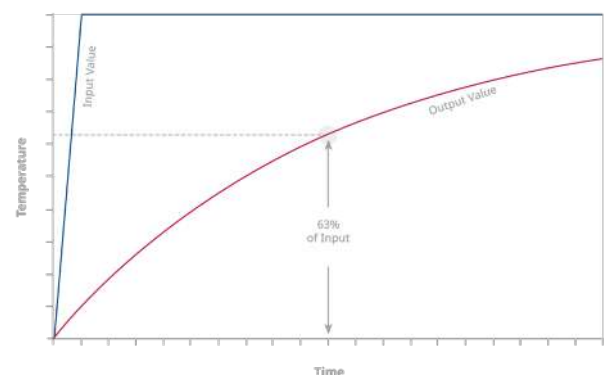
Figure 3-15: Damping Response Curve
