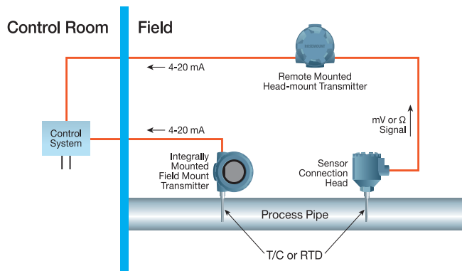
Figure 4-29: Installation Options
