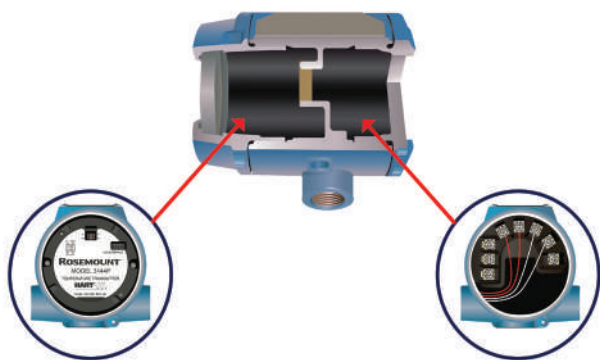
Figure 6-1: Dual Compartment Housing
