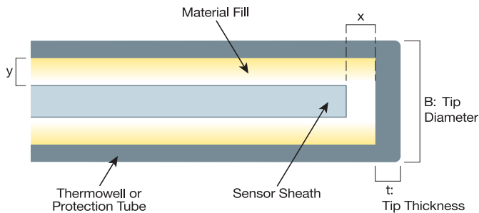
Figure 3-59: Factors Affecting Response Time
