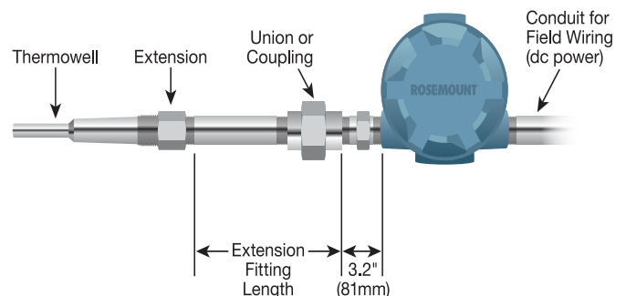
Figure 4-33: Typical North American Mounting
