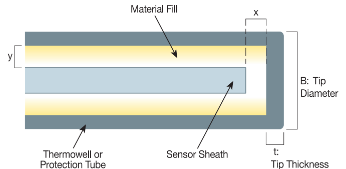
Figure 3-83: Factors Affecting Response Time for a Large Bore Thermowell
