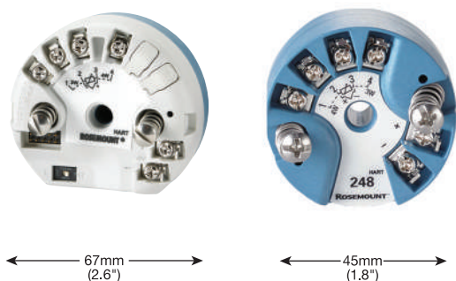
Figure 3-25: DIN A and DIN B Head Mount Housing Styles
