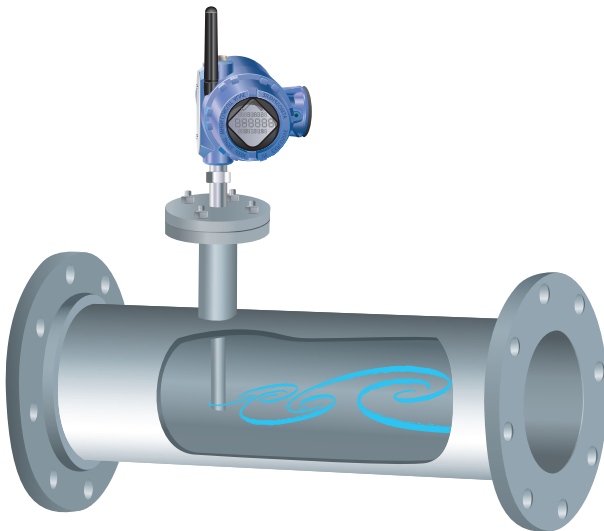
Figure 3-54: Wireless Integral Mount Pipeline Installation
