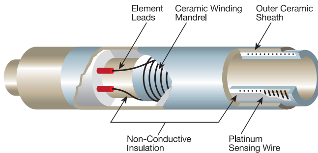
Figure 3-46: Mandrel Style Wire-Wound Element
