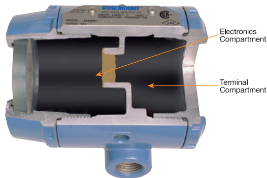
Figure 4-20: Dual-Compartment Housing
