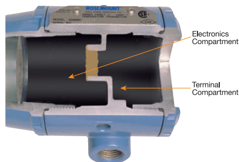
Figure 3-28: Dual-Compartment Housing
