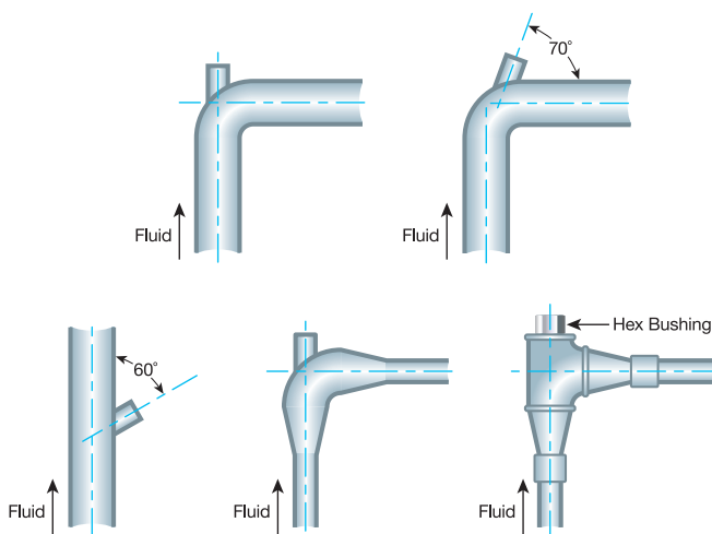
Figure 4-7: Thermowell Angled Installation Options
