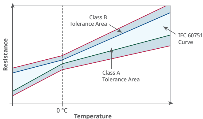
Figure 3-63: IEC 60751 Ideal vs. Class A vs. Class B Tolerance Bands
