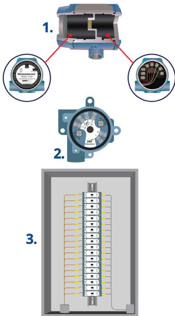
Figure 3-1: Transmitter Styles (from top to bottom): 1.) Field Mount, 2.) Head Mount, 3.) Rail Mount
