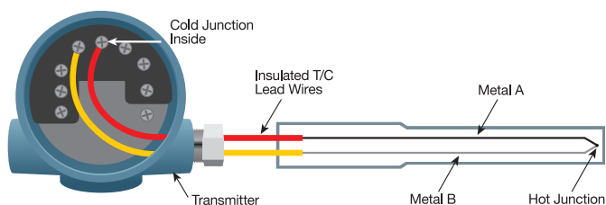
Figure 3-71: Cold Junction Compensation
