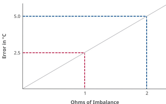
Figure 3-45: Lead Imbalance vs. Error for 3-Wire RTD
