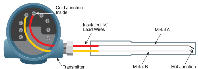
Figure 3-9: Cold Junction Compensation
