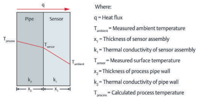
Figure 3-107: Simplified Heat Flux through a Pipe and Temperature Sensor Installation
