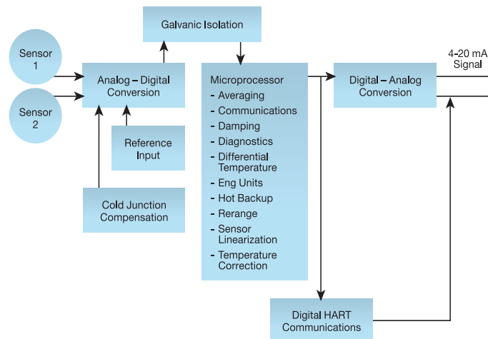
Figure 3-2: Transmitter Functional Block Diagram
