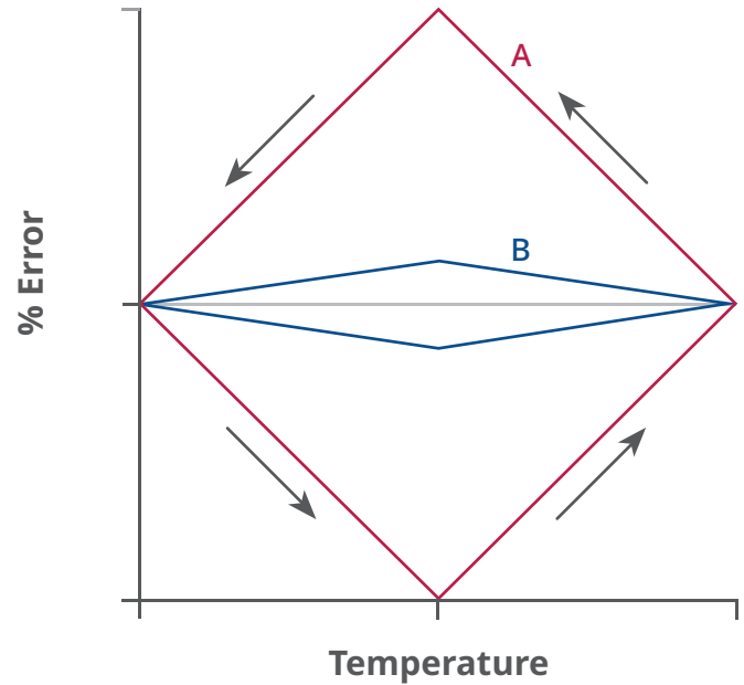
Figure 3-60: Hysteresis for Thin Film (A) and for Helical Coil Wire-Wound Elements (B)
