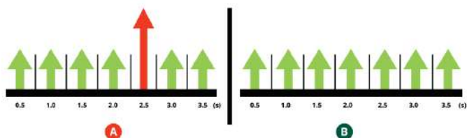
Figure 3-16: Output Without Open Sensor Holdoff (A) and With Open Sensor Holdoff (B)
