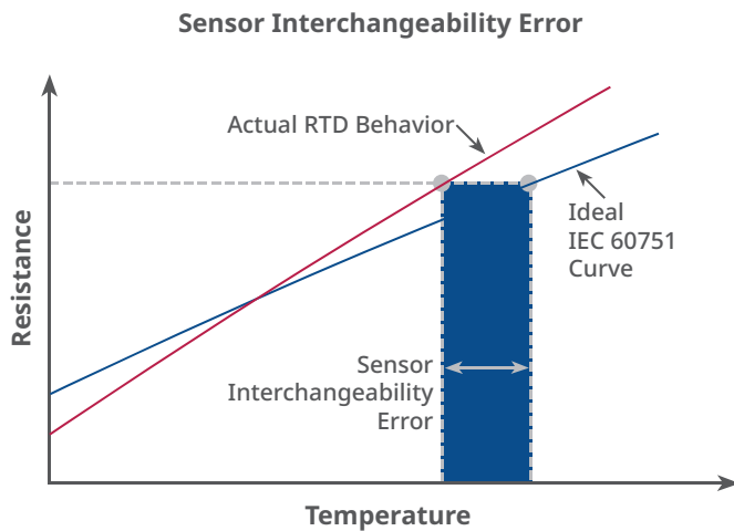
Figure 3-66: Sensor Interchangeability Error
