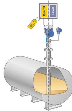
FMCW Radar 2-in-1
