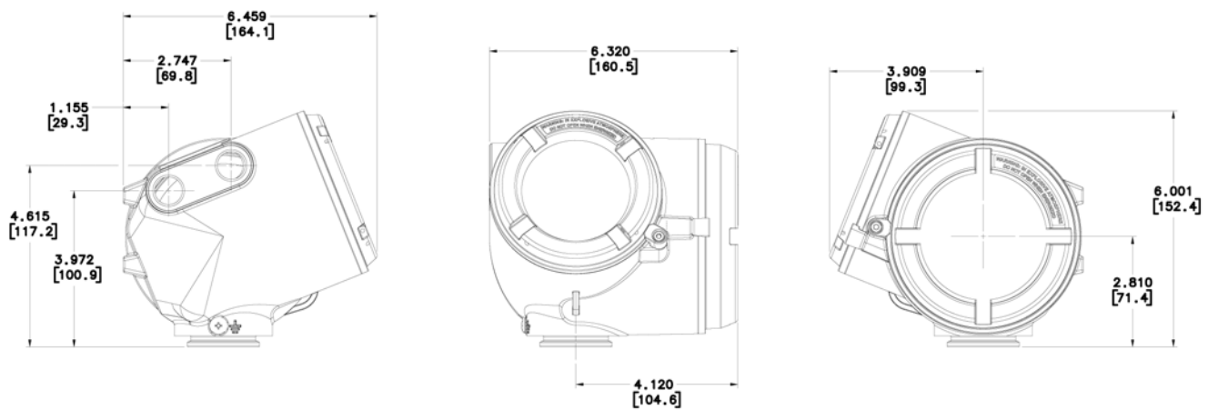
Figure 1: 4700 Transmitter - Aluminum Painted Housing Integral Installation
