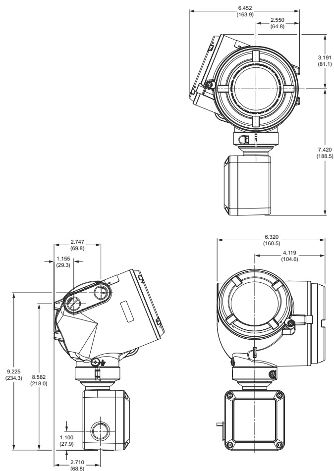
Figure 2: 4700 Transmitter - Aluminum Painted Housing Remote Installation
