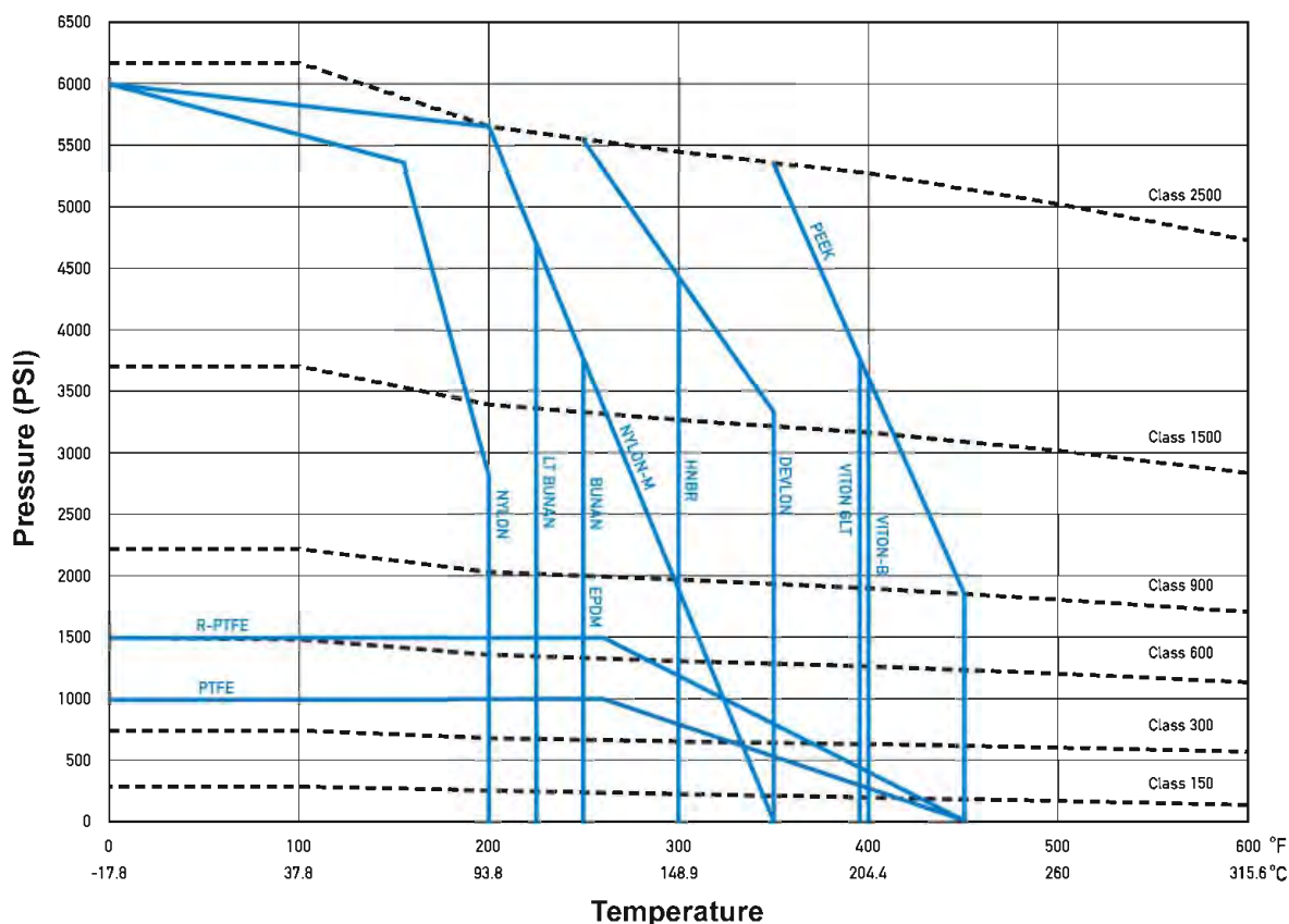
Pressure-Temperature Chart
