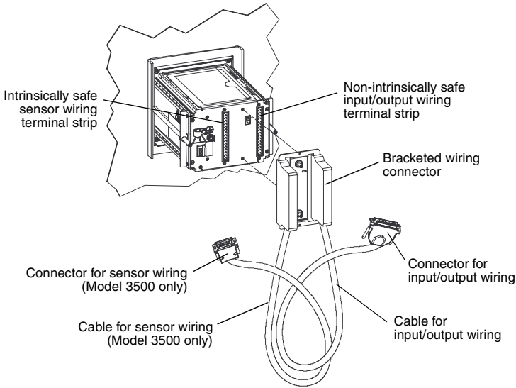
Figure 7. Wiring connectors and terminals – I/O cables
