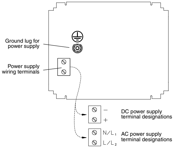
Figure 13. Power supply wiring terminals
