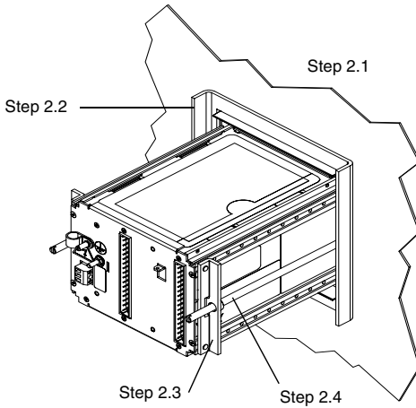
Figure 4. Steps for installation in panel
