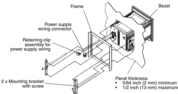
Figure 1. Panel-mount installation kit
