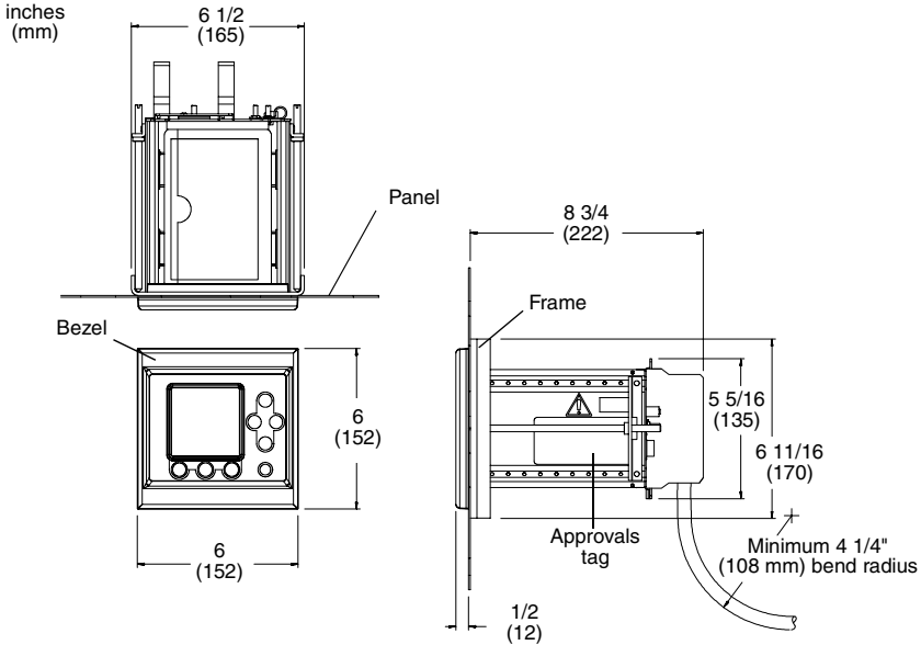
Figure 3. Panel-mount dimensions – I/O cables
