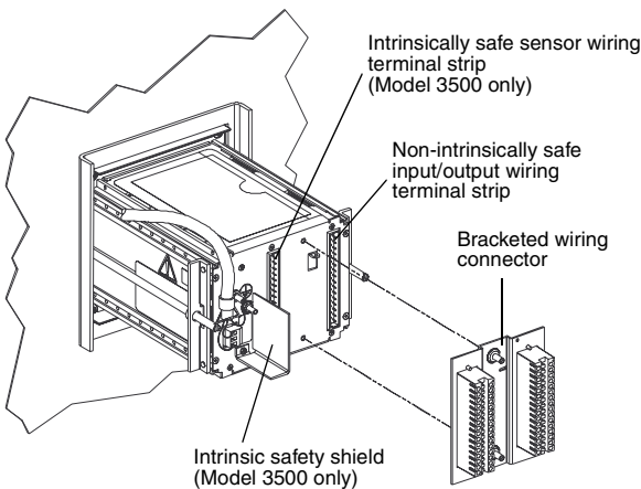
Figure 5. Wiring connectors and terminals – screw-type connectors
