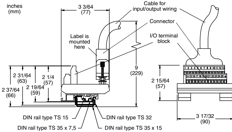
Figure 8. Installing terminal block for I/O wiring on DIN rail
