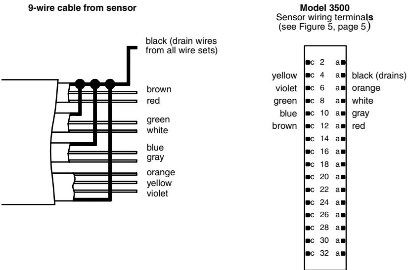
Figure 10. Sensor cable to Model 3500 – screw-type connectors
