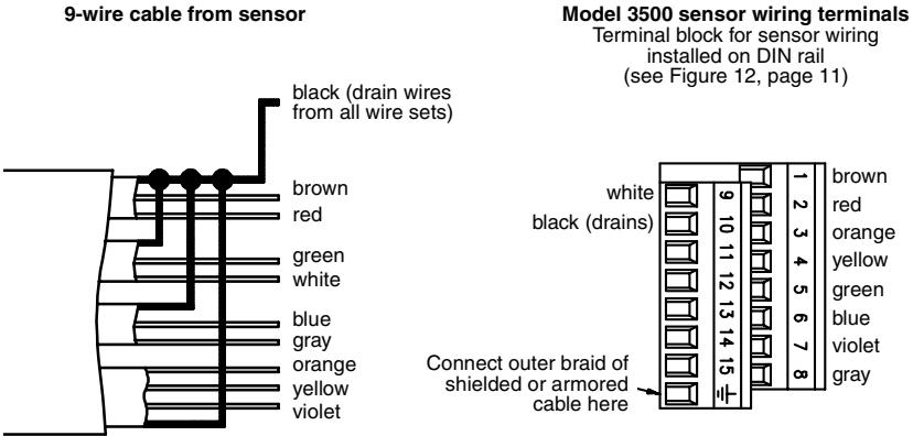
Figure 11. Sensor cable to Model 3500 – I/O cables
