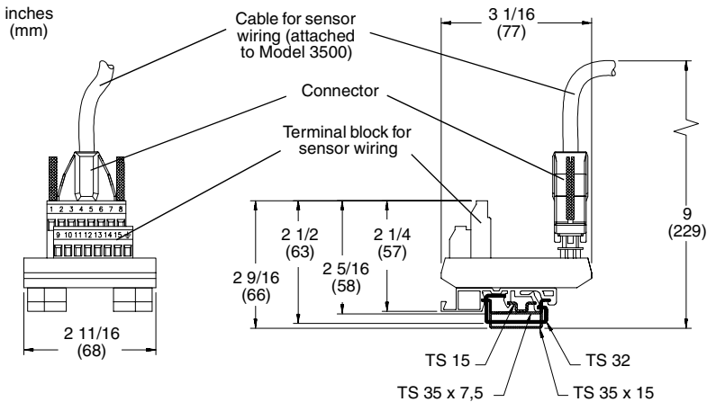
Figure 12. Installing terminal block for sensor wiring on DIN rail
