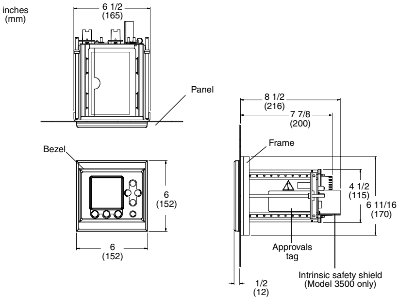
Figure 2. Panel-mount dimensions – screw-type connectors
