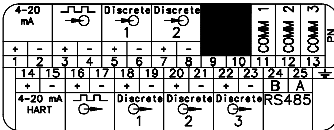
Figure 9. Input/output wiring terminal card – I/O cables
